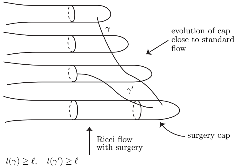
FIGURE 2. Paths in evolving surgery caps are long.
