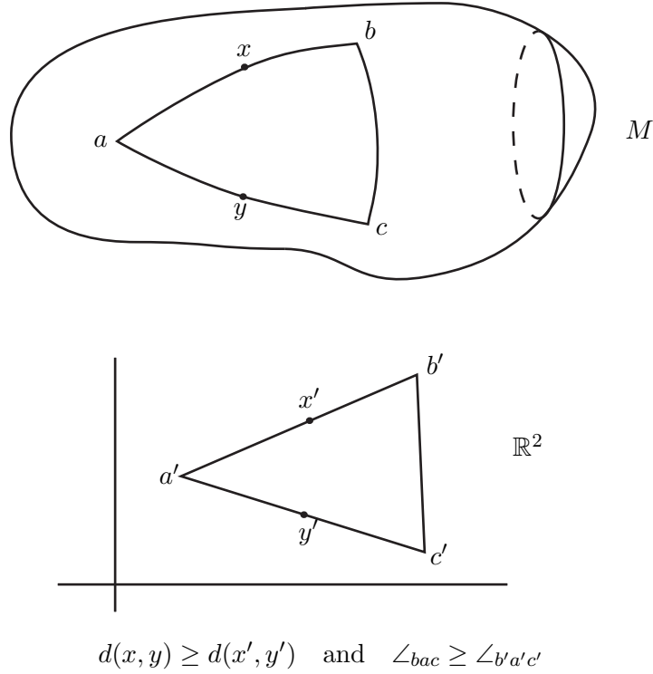
FIGURE 1. Toponogov comparison.
