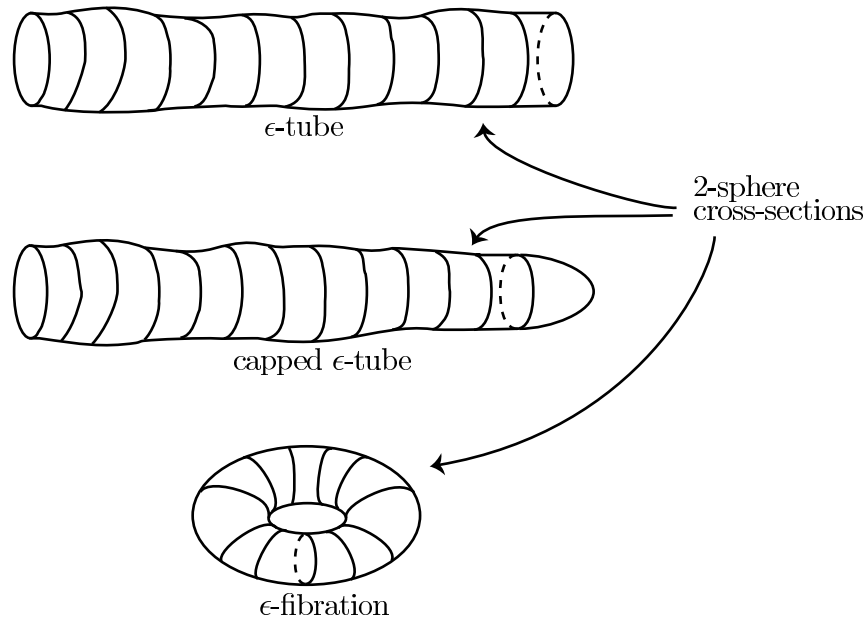
FIGURE 2. \epsilon -canonical neighborhoods.
