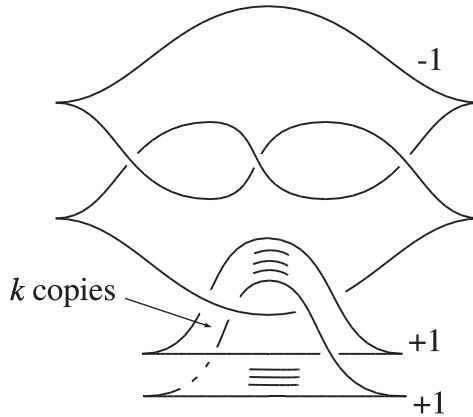
FIGURE 5. Equivalent surgery diagram for (V_k, \xi_k)
