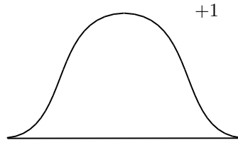
FIGURE 4. A contact structure with nonvanishing invariant
