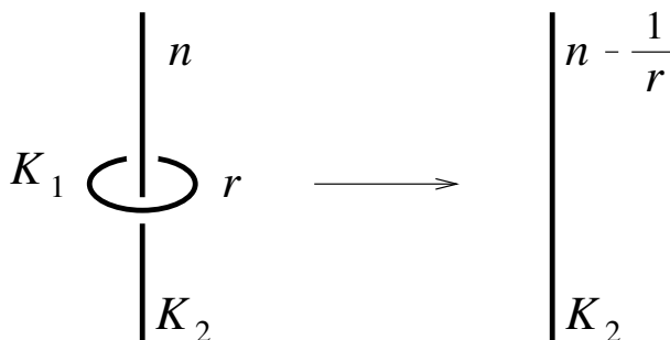
FIGURE 3. The slam-dunk operation
