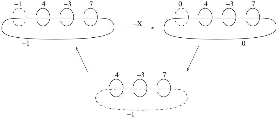
FIGURE 11. The exact triangle induced by -X
