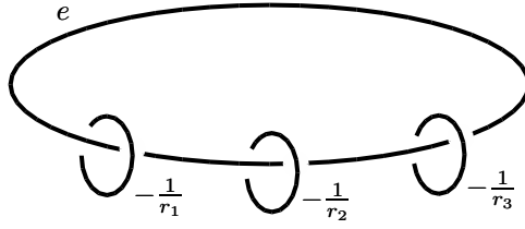
FIGURE 7. Another diagram for the small Seifert fibered 3-manifold M
