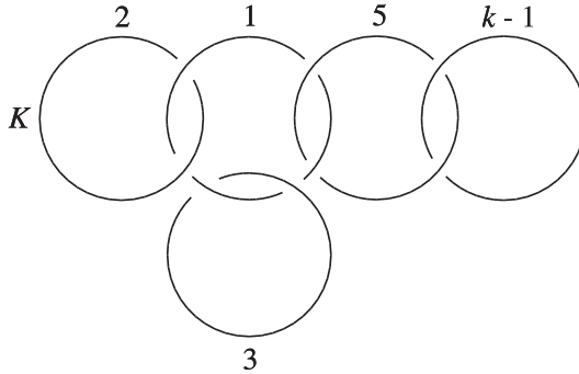
FIGURE 6. A surgery diagram for -V_k
