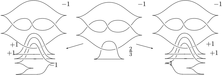
FIGURE 2. Two contact structures on Y_3(T)
