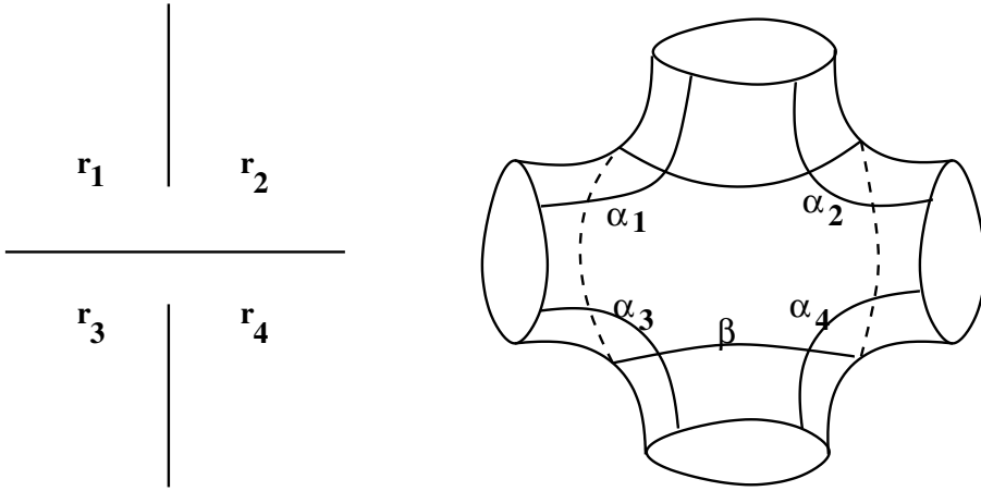
FIGURE 10. Special Heegaard diagram for knot crossings. At each crossing as pictured on the left, we construct a piece of the Heegaard surface on the right (which is topologically a four-punctured sphere). The curve \beta is the one corresponding to the crossing on the left; the four arcs \alpha_1, \dots, \alpha_4 will close up.
