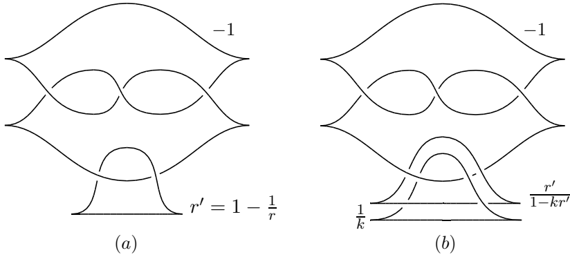
FIGURE 3. Surgery diagrams for contact structures on Y_r(T)
