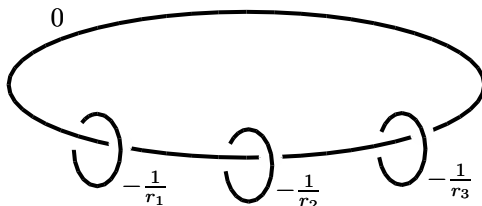
FIGURE 2. Surgery diagram for the Seifert fibered 3-manifold M(r_1, r_2, r_3)
