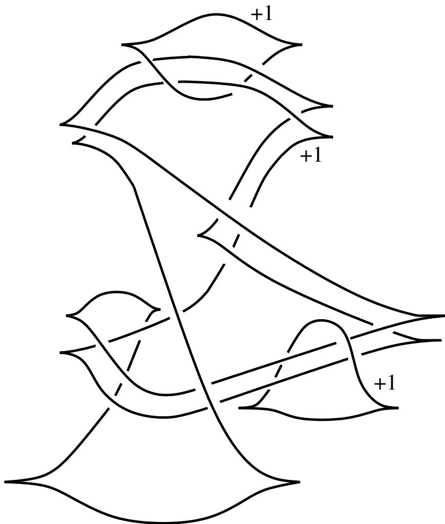
FIGURE 12. Nonfillable tight contact circle bundle
