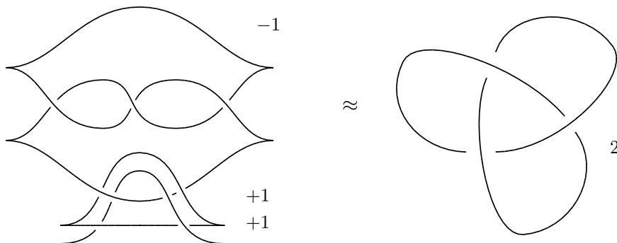
FIGURE 1. A contact structure on Y_2(T)
