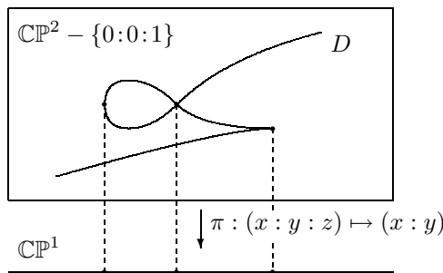
FIGURE 1. A Hurwitz curve in \mathbb{CP}^2
