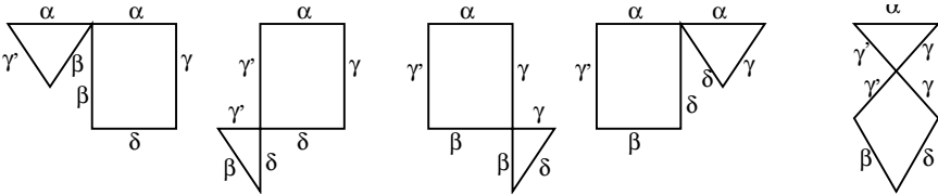
FIGURE 7. Degenerate pentagons. We have illustrated here a schematic diagram for the degenerations of pseudo-holomorphic pentagons. We have dropped the five additional degenerations, where a Whitney disk bubbles off the vertex of any pentagon.
