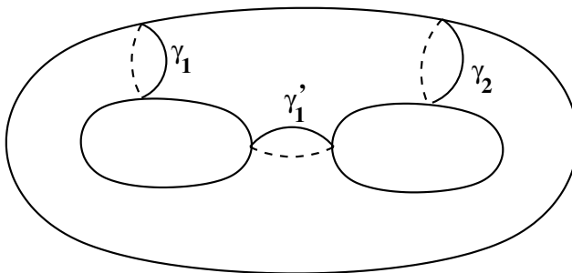
FIGURE 3. Handlesliding \gamma_1 over \gamma_2 .
