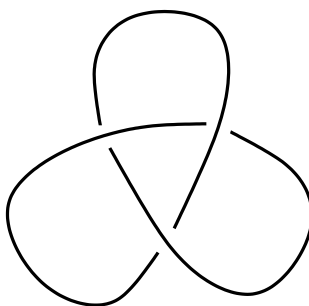
FIGURE 8. The right-handed trefoil knot
