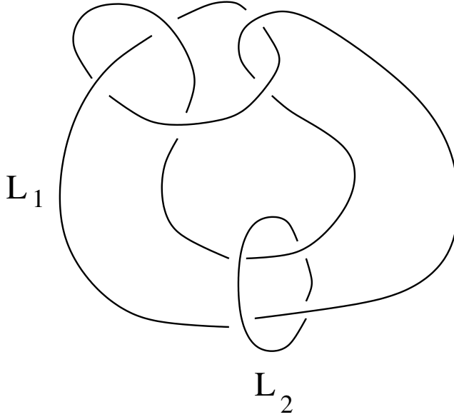
FIGURE 10. A two-component link. Each component is unknot -ted; blowing down either one or the other component gives a pair of distinct knots K_1 and K_2 in S^3 with S^3_{-1}(K_1) \cong S^3_{-1}(K_2) .
