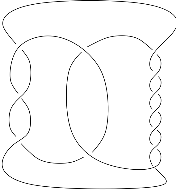
FIGURE 2. The (-2, 3, 7) pretzel knot. Surgery on this knot with coefficients 18 and 19 give the lens spaces L(18, 5) and L(19, 8) respectively.
