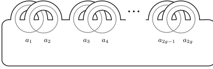
FIGURE 16. The curves a_1, \dots, a_{2g} on \Sigma .
