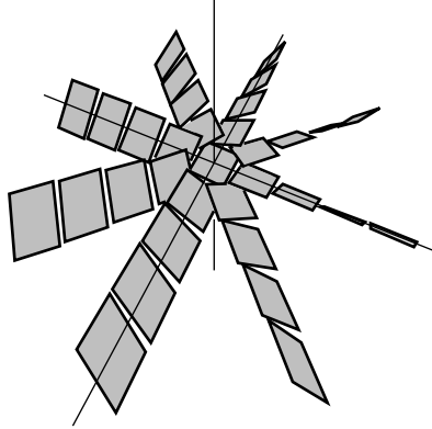
FIGURE 7. The standard contact structure on \mathbb{R}^3 . (Picture by Stephan Schönenberger.)
