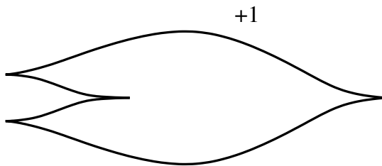
FIGURE 4. Contact structure \xi_1 on S^3
