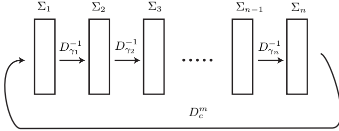
FIGURE 15. Breaking up the monodromy.
