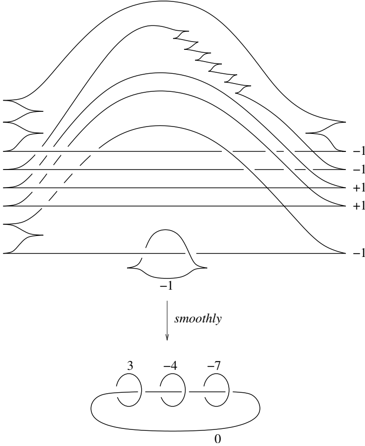
FIGURE 10. Tight contact structure on Y = M(-\frac{1}{2}, \frac{1}{4}, \frac{1}{7}) = S_5^3(T_{(3,4)})
