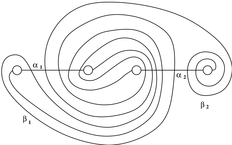
FIGURE 2. A genus 2 Heegaard diagram.
