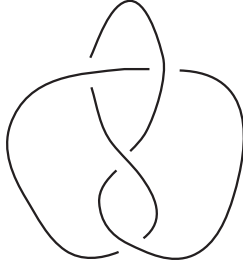
FIGURE 12. The figure eight knot
