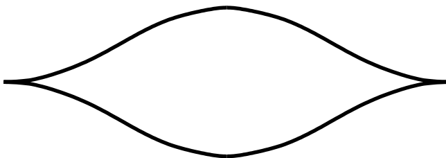
FIGURE 6. The Legendrian unknot
