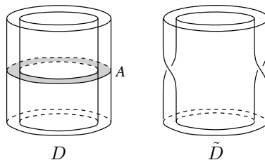
FIGURE 2. The braiding construction
