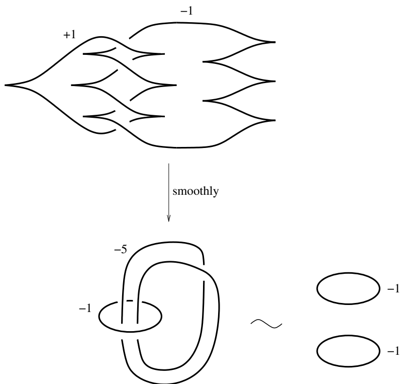
FIGURE 5. Contact structure \xi_{-1} on S^3
